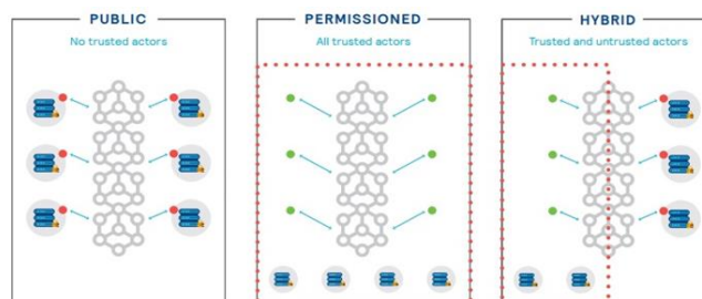
Figure 2. Types of Block Chain Networks.
